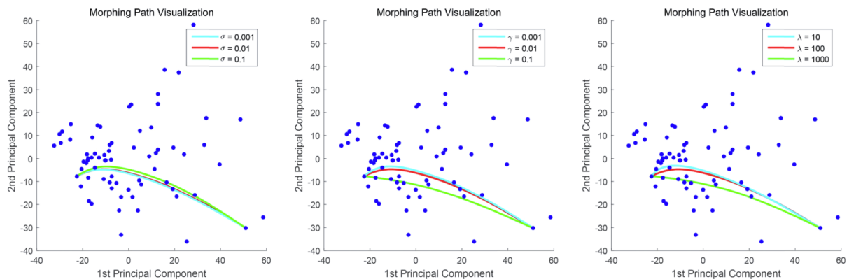
Figure 6: Visualization of the morphing paths with varying parameters. (Left) Changing \sigma to 0.001, 0.01 (default) and 0.1; (middle) changing \gamma to 0.001, 0.01 (default) and 0.1; (right) changing \lambda to 10, 100 (default) and 1000.
