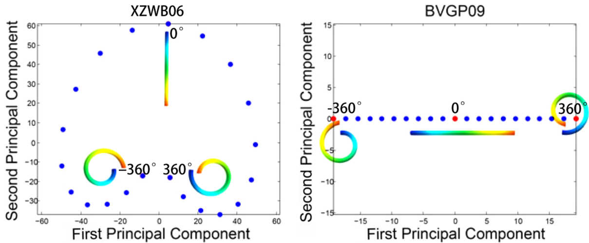
Figure 4: Visualization of blended cylinder from -360^\circ to 360^\circ using dimensionality reduction to 2D. (Left) Result of Poisson shape interpolation [XZWB06], (right) result of [BVGP09].
